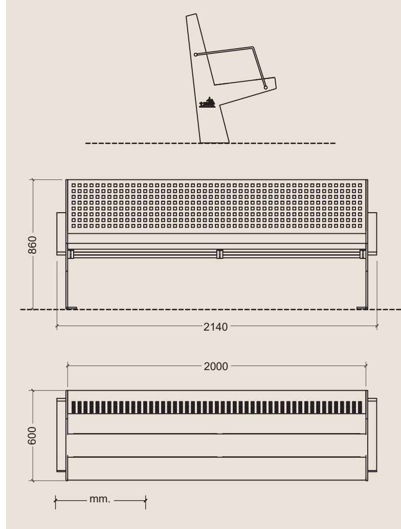
BANCO RUZAFÁ 200 MIXTO BENCH "RUZAFÁ" 200 CM, MIXED BANC "RUZAFÁ" 200 CM, MIXTE
